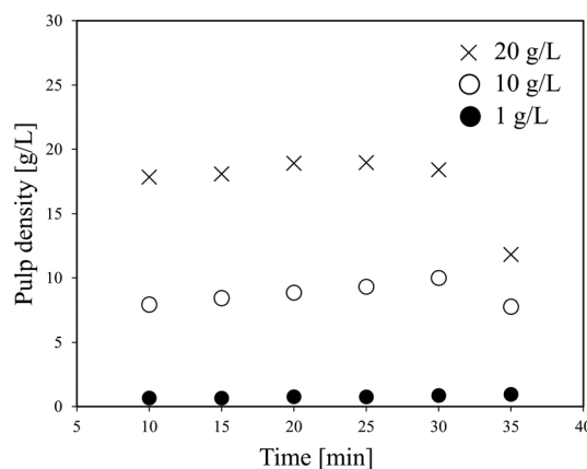
Fig. 3 Effect of time on the pulp density of the recovered solution using flow line B (LiCoO 2 , 30 ml min -1 ).
