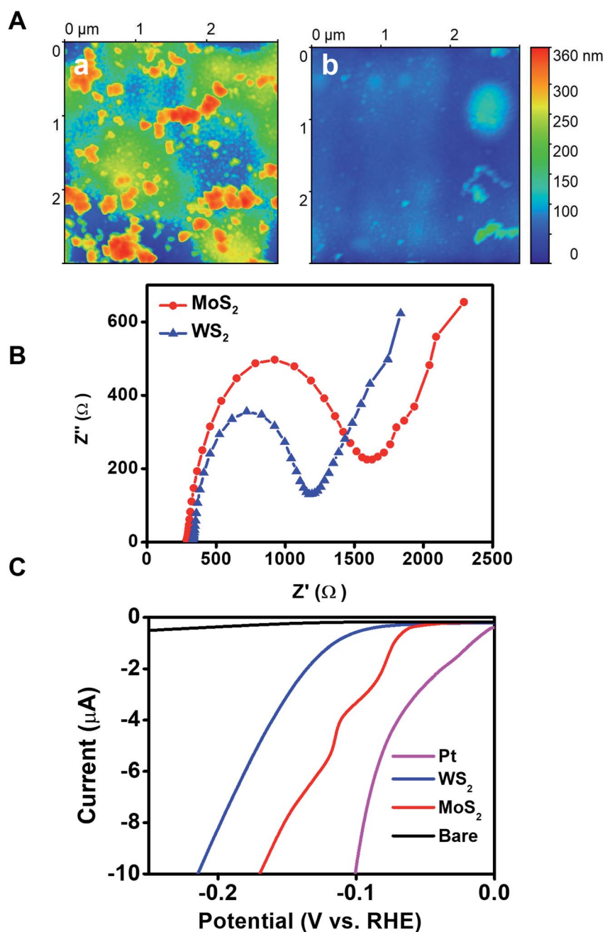
Fig. 3 Surface morphology and catalytic activity of \text{WS}_2/\text{Ni}/\text{Pt} micromotors. (A) AFM topographical images showing the surface morphology of (a) \text{WS}_2/\text{Ni}/\text{Pt} and (b) \text{MoS}_2/\text{Ni}/\text{Pt} control micromotors. Images were processed with Gwyddion software to subtract the micromotor curvature to better display the morphology at the nanometer level. (B) Nyquist plots and (C) linear sweep voltammograms of \text{WS}_2/\text{Ni}/\text{Pt} and \text{MoS}_2/\text{Ni}/\text{Pt} microtube-modified electrodes. For the Nyquist plots, \text{Fe}(\text{CN})_6^{4-/3-} is used as a redox probe.
