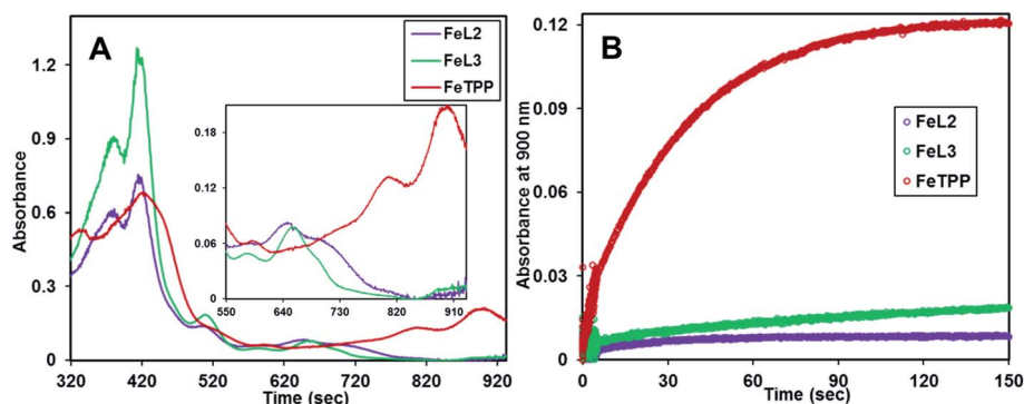
Fig. 5 Rapid-scan electronic absorption spectra of the reaction of iron porphyrin complexes (50 \mu M) with 8 equivalent of meta -chloroperbenzoic acid ( m -CPBA, 200 \mu M) in dichloromethane followed at -30 °C. (A) Selected overlay spectra representing the intermediate species formed after 50 s of the reaction, (B) overlay of the time traces at the 900 nm band with the formation of isoporphyrin species ( \lambda_{\text{max}} = 900 nm) for these three complexes (Fe III TPP(Br) (red line), Fe III L2(Br) (violet line) and Fe III L3(Br) (green line)).
