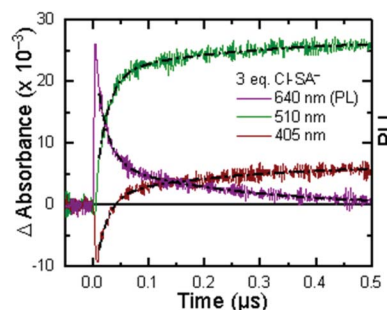
Fig. 9 Single wavelength transient absorption kinetics monitored at 405 nm, red, and 510 nm, green, for [\text{Ru-LL}^{4+}, \text{Cl-SA}^-]^{3+} . The purple trace is the excited-state decay. Overlaid in black are biexponential fits with the two lifetimes shared between the three traces. The negative signal is due to small amounts of excited-state bleach still present of the monitored wavelengths.
