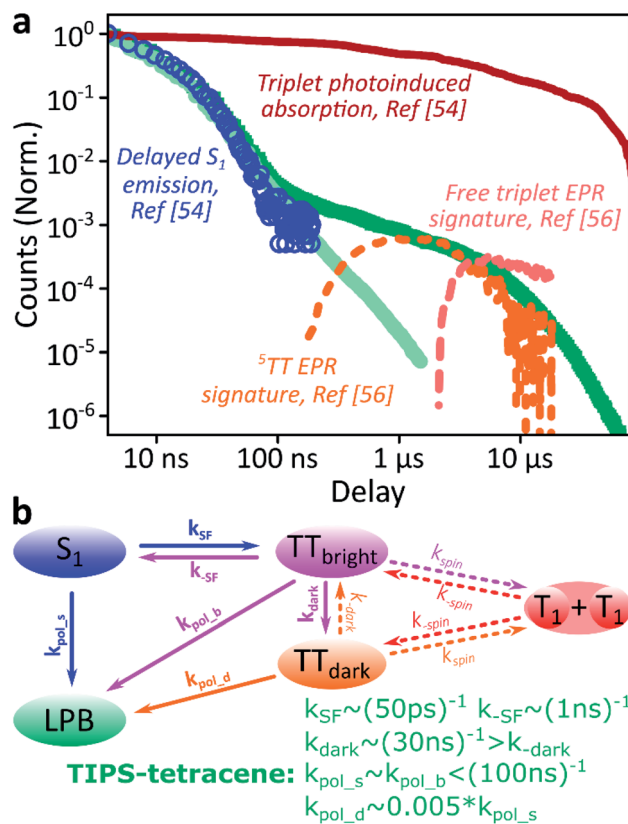
Fig. 5 Identification of the {}^5\text{TT} contribution. (a) Reproduction of the TIPS-tetracene film and microcavity emission kinetics from Fig. 4d, compared with time-correlated single photon counting (circles, ref. 54), transient absorption (solid, ref. 54) and electron paramagnetic resonance (dashed, ref. 56) kinetics previously reported for equivalent polycrystalline films. The long-time enhancement in microcavities coincides with observations of high-spin {}^5(\text{TT}) . (b) Rate model used to describe dynamics within the exciton reservoir. \text{TT}_{\text{bright}} are triplet-pair states that directly mix with \text{S}_1 . \text{TT}_{\text{dark}} states are unable to efficiently repopulate \text{S}_1 . Rates shown are from fitting to published data. A similar model would describe diphenylanthracene: PtOEP or DPPT, replacing k_{\text{SF}} with k_{\text{ISC}} directly to the (single) triplet states and including the effects of exciton diffusion within k_{\text{spin}} . Nonradiative decay (from all states) and radiative decay (from \text{S}_1 , LPB) omitted for clarity.
