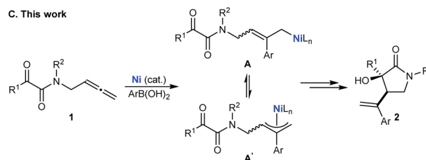
Scheme 1 Nickel-catalyzed arylyative cyclizations of allenes.
