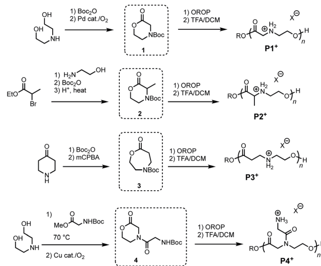
Fig. 2 Synthesis of azalactone monomers and polymers.
