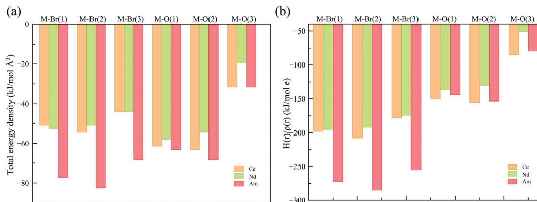
Fig. 6 (a) Total energy density over the electron density (b) total energy density over concentration of electron density at the BCP derived from a SR-CAS(7,7) wave function. See ESI† for exact numbers.
