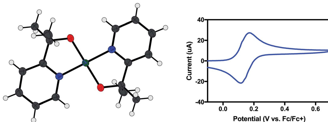
Fig. 1 (Left) X-ray crystal structure of \text{Ni}(\text{pyalk})_2 ( 1 ). Atoms are shown at the 50% probability level ( 1 ). (Right) Cyclic voltammogram of 1 in \text{MeCN} . The reversible wave at 0.15 V vs. \text{Fc}/\text{Fc}^+ is assigned as a \text{Ni}^{\text{II/III}} couple.
