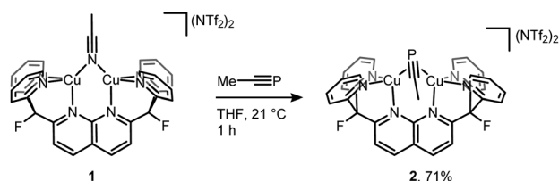
Scheme 1 Synthesis of [\text{Cu}_2(\mu\text{-}\eta^2:\eta^2\text{-MeCP})\text{DPFN}](\text{NTf}_2)_2 ( 2 ).
