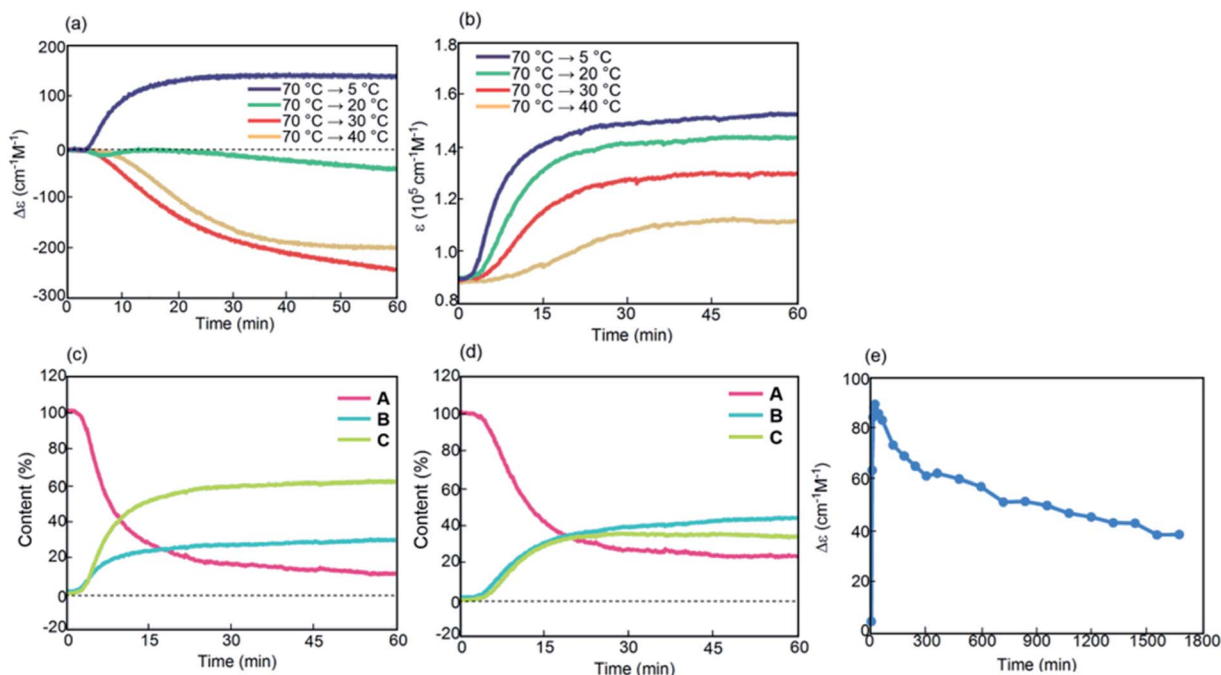
Fig. 4 Kinetic analysis under isothermal conditions of (P)-1-C 16 /(M)-2 in fluorobenzene (0.5 mM) shown using (a) \Delta\epsilon(314\text{ nm})/\text{time} profiles and (b) \epsilon(314\text{ nm})/\text{time} profiles at 5, 20, 30, and 40 °C for 60 min. Content/time profiles are also shown at (c) 5 °C and (d) 20 °C. (e) A long experiment was conducted at 5 °C as shown using \Delta\epsilon(314\text{ nm})/\text{time} profiles.
