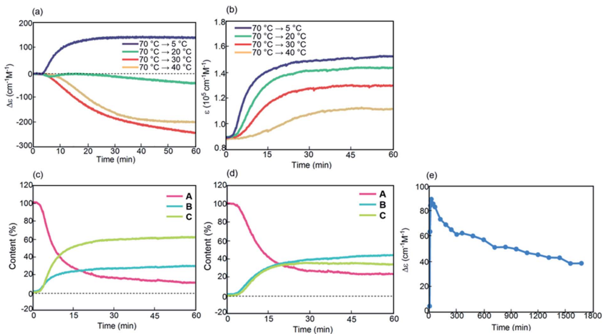
Fig. 4 Kinetic analysis under isothermal conditions of (P)-1-C 16 /(M)-2 in fluorobenzene (0.5 mM) shown using (a) \Delta\epsilon (314 nm)/time profiles and (b) \epsilon (314 nm)/time profiles at 5, 20, 30, and 40 °C for 60 min. Content/time profiles are also shown at (c) 5 °C and (d) 20 °C. (e) A long experiment was conducted at 5 °C as shown using \Delta\epsilon (314 nm)/time profiles.
