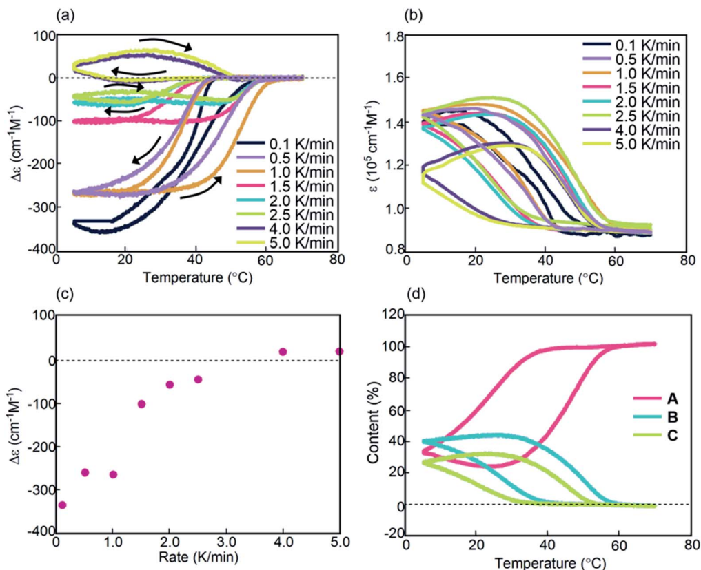
Fig. 3 Experiments on cooling and heating at constant rates between 0.1 and 5.0 K min -1 using (P)-1-C 16 /(M)-2 in fluorobenzene (0.5 mM), as shown using (a) \Delta\epsilon (314 nm)/temperature and (b) \epsilon (314 nm)/temperature profiles. Temperature was decreased from 70 to 5 °C and then increased from 5 °C to 70 °C. (c) Profiles of \Delta\epsilon (314 nm) at 5 °C as a function of cooling rate. (d) Content/temperature profiles at 2.0 K min -1 .
