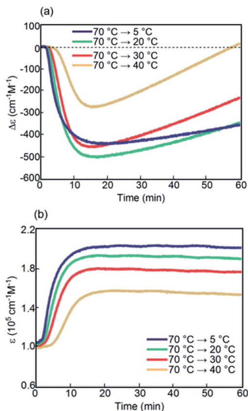
Fig. 10 (a) \Delta\epsilon (314 nm)/time profiles and (b) \epsilon (314 nm)/time profiles for ( P )-1/ (M) -2 in fluorobenzene (0.5 mM) at 5, 20, 30, and 40 °C.
