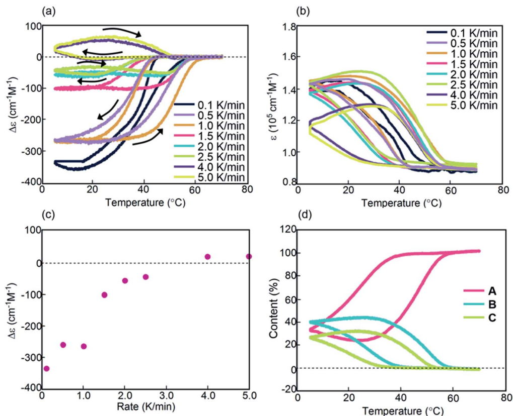
Fig. 3 Experiments on cooling and heating at constant rates between 0.1 and 5.0 K min -1 using (P)-1-C 16 /(M)-2 in fluorobenzene (0.5 mM), as shown using (a) \Delta\epsilon(314\text{ nm})/\text{temperature} and (b) \epsilon(314\text{ nm})/\text{temperature} profiles. Temperature was decreased from 70 to 5 °C and then increased from 5 °C to 70 °C. (c) Profiles of \Delta\epsilon(314\text{ nm}) at 5 °C as a function of cooling rate. (d) Content/temperature profiles at 2.0 K min -1 .
