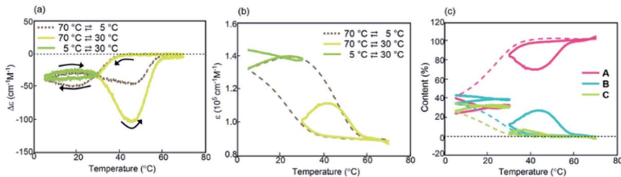
Fig. 5 (a) \Delta\epsilon(314\text{ nm}) /temperature profiles and (b) \epsilon(314\text{ nm}) /temperature profiles of (P) -1- C_{16}/(M) -2 in fluorobenzene (0.5 mM) at a cooling and heating rate of 2.0\text{ K min}^{-1} . The temperature was decreased from 70\text{ }^{\circ}\text{C} to 30\text{ }^{\circ}\text{C} and then increased to 70\text{ }^{\circ}\text{C} (yellow lines); the temperature was decreased from 70\text{ }^{\circ}\text{C} to 5\text{ }^{\circ}\text{C} , increased to 30\text{ }^{\circ}\text{C} , and then decreased to 5\text{ }^{\circ}\text{C} (green lines). (c) Content/temperature profiles are also shown. Dashed lines were obtained from Fig. 3a and d during cooling.
