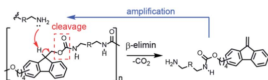
Scheme 2 Degradation mechanism of base-triggered self-amplifying degradable polyurethane.
