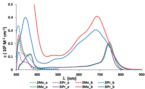
Fig. 1 Absorption spectra of 10^{-5} M 2^{\text{Mea-b}} and 2^{\text{iPra-b}} (dashed line) and 3^{\text{Mea-b}} and 3^{\text{iPra-b}} (solid line) in \text{CH}_2\text{Cl}_2 at 25^\circ\text{C} .
