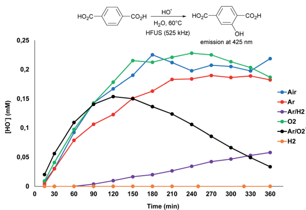
Scheme 3 Titration of \text{OH}^\bullet radical using TPA (2 mM) as a function of the gaseous atmosphere. *The decrease in the \text{OH}^\bullet radical amount with time under Ar/ \text{O}_2 is due to the large production of \text{OH}^\bullet radicals which degrade TPA-OH used as a probe.
