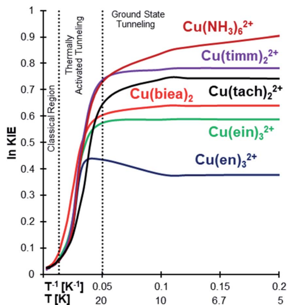
Fig. 4 ln KIE vs. T^{-1} for \text{Cu}(\text{II})\text{-N}_6 type complexes in the gas phase for ^{14}\text{N}/^{15}\text{N} substitution in all the nitrogens. All the complexes are showing a large KIE at low temperatures.
