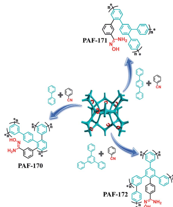
Fig. 1 Scheme of synthesis for PAF-AOs: \text{AlCl}_3/\text{CHCl}_3 , 60 \text{ }^\circ\text{C} , 48 \text{ h} . \text{NH}_2\text{OH} \cdot \text{HCl}/\text{N}(\text{CH}_2\text{CH}_3)_3/\text{EtOH} , 70 \text{ }^\circ\text{C} , 48 \text{ h} .
