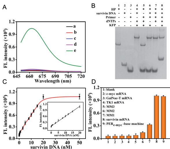
Fig. 2 (A) Fluorescence responses of the activable PER based-DNA machine to target mRNA. (a) 200 nM primers + 20 nM survivin DNA + 200 μM dNTPs + 25 U mL -1 KFP + 30 nM MB; (b) 20 nM HP + 20 nM survivin DNA + 200 μM dNTPs + 25 U mL -1 KFP + 30 nM MB; (c) 20 nM HP + 200 nM primers + 20 nM survivin DNA + 25 U mL -1 KFP + 30 nM MB; (d) 20 nM HP + 200 nM primers + 20 nM survivin DNA + 200 μM dNTPs + 30 nM MB; and (e) 20 nM HP + 200 nM primers + 20 nM survivin DNA + 200 μM dNTPs + 25 U mL -1 KFP + 30 nM MB. (B) Corresponding to polyacrylamide gel electrophoresis (PAGE) of the PER based-DNA machine as mentioned above. (C) Relationship between the fluorescence intensities at 665 nm and the concentrations of the survivin DNA target from 0 to 50 nM. Insert: linear correlation between fluorescence intensities and survivin DNA concentrations in the range of 0.005–20 nM. (D) Specificity of the survivin DNA initiated PER-based DNA machine.
