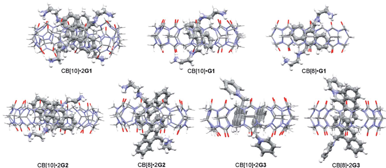
Fig. 4 Plausible binding modes of guests with CB[ n ] (MMFF-minimized).
