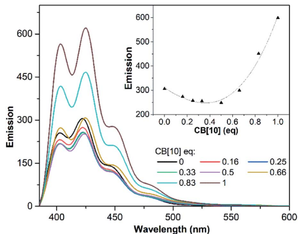
Fig. 3 Fluorescence emission spectra recorded for G1 (31.25 \mu\text{M} ) upon titration with CB[10]. Inset: emission of G1 vs. CB[10] equivalent ( \lambda_{\text{ex}} = 250 nm, \lambda_{\text{em}} = 422 nm).
