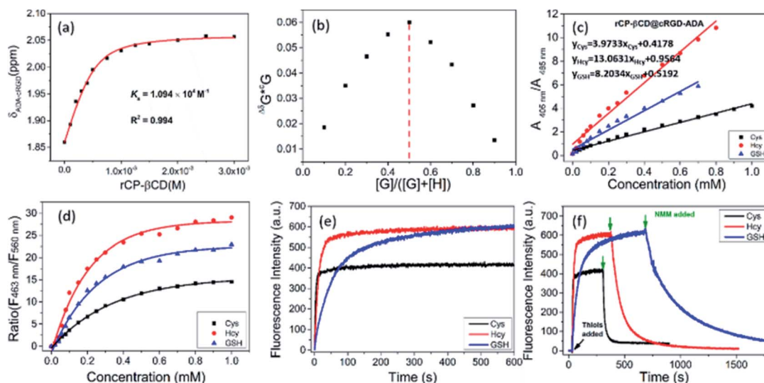
Fig. 3 Construction of rCP- \beta CD@cRGD-ADA and reaction efficiency towards biothiols. (a) Nonlinear least-squares fit of the change in chemical shift of the cRGD-ADA (0.5 mM) peaks at \delta = 1.86 ppm as a function of rCP- \beta CD concentration (0–3 mM). (b) Job's plot of cRGD-ADA (G) and rCP- \beta CD (H) in D 2 O ([cRGD-ADA] + [rCP- \beta CD] = 2 mM) at 25 °C. (c) Plots of UV-vis absorption peak ratios ( A_{405\text{ nm}}/A_{485\text{ nm}} ) for rCP- \beta CD@cRGD-ADA (10 \mu M) as a function of biothiol concentration (0–1 mM) in PBS. (d) Dose–response curves for the reactions of rCP- \beta CD with biothiols (0–1 mM). (e) Time-dependence of the fluorescence emission at 463 nm for rCP- \beta CD@cRGD-ADA in response to biothiols (0.5 mM). (f) Time-dependence of the reversible fluorescence emission at 463 nm for rCP- \beta CD in response to biothiols (0.5 mM) and NMM (0.5 mM) ( \lambda_{\text{ex}} = 405 nm; slits: 2.5/5 nm).
