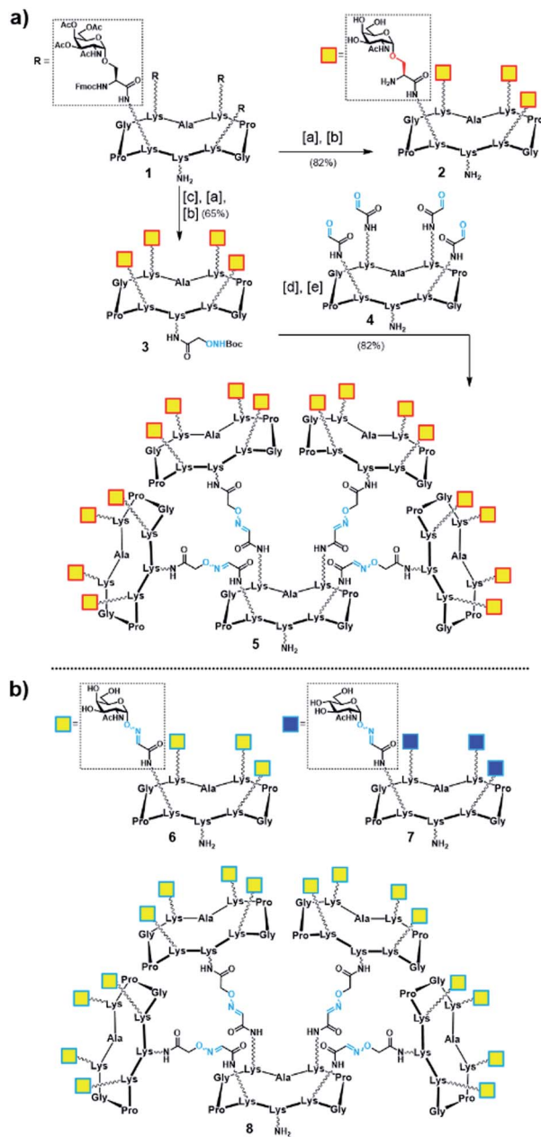
Scheme 1 (a) Synthesis of tetra- and hexadeca-valent Tn-Ser glycodendrimers 2 and 5 . Reagents and conditions: [a] 5% piperidine in \text{CH}_3\text{CN} , r.t., 15 min; [b] \text{NaOMe}/\text{MeOH} (pH \approx 10), r.t., 20 min; [c] Boc-Aoa-NHS (1.2 eq.), DIPEA (2.0 eq.), \text{CH}_3\text{CN}/\text{DMF} (1 : 1), 20 min; [d] TFA/ \text{CH}_2\text{Cl}_2 (1 : 1), r.t., 30 min; [e] 4 (ref. 72) (0.17 eq.), 0.1% TFA in \text{H}_2\text{O} , 37 °C, 45 min. (b) Tn-oxime glycodendrimers 6 (ref. 61) and 8 (ref. 73), and tetra-valent GlcNAc-oxime control 7 (ref. 73).
