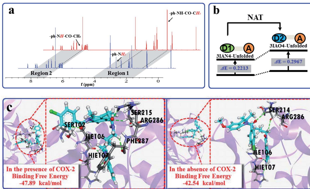
Fig. 3 (a) The 1 H NMR spectra changes of 3IAN4 with NAT under acetyl-CoA. (b) Simple diagram of energy difference ( \Delta E ) of 3IAN4- Unfolded and 3IAO4- Unfolded . (c) The molecular dynamics calculation results and the binding free energies for the reaction between 3IAN4 and NAT (PDB ID: 1BM0) in the presence and absence of COX-2 (PDB ID: 3NT1).
