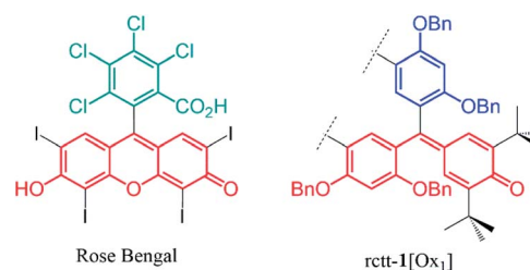
Fig. 5 Chemical structures of Rose Bengal (left) and the chromophore moiety of the structure of rctt-1[Ox 1 ] reveals a similar hemiquinonoid conjugated with electron rich aromatic substituents in the chromophore structure.
