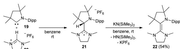
Scheme 2 Formal CH insertion of 19 and deprotonation afforded 22 .
