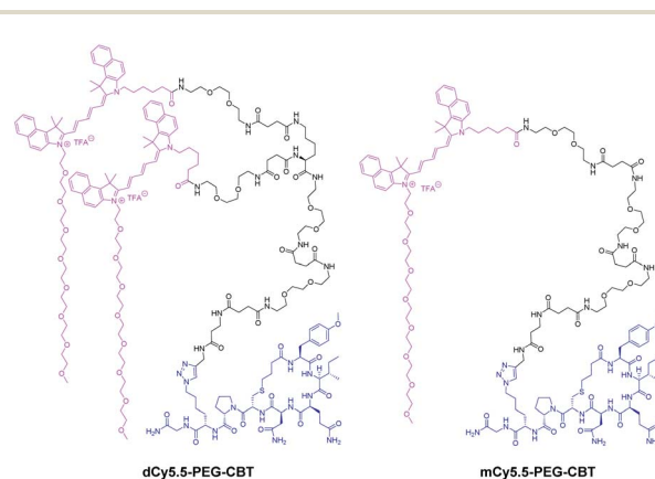
Fig. 2 Structures of the conjugates of the NIR fluorogenic dimer and the corresponding monomer with the carbetocin ligand.
