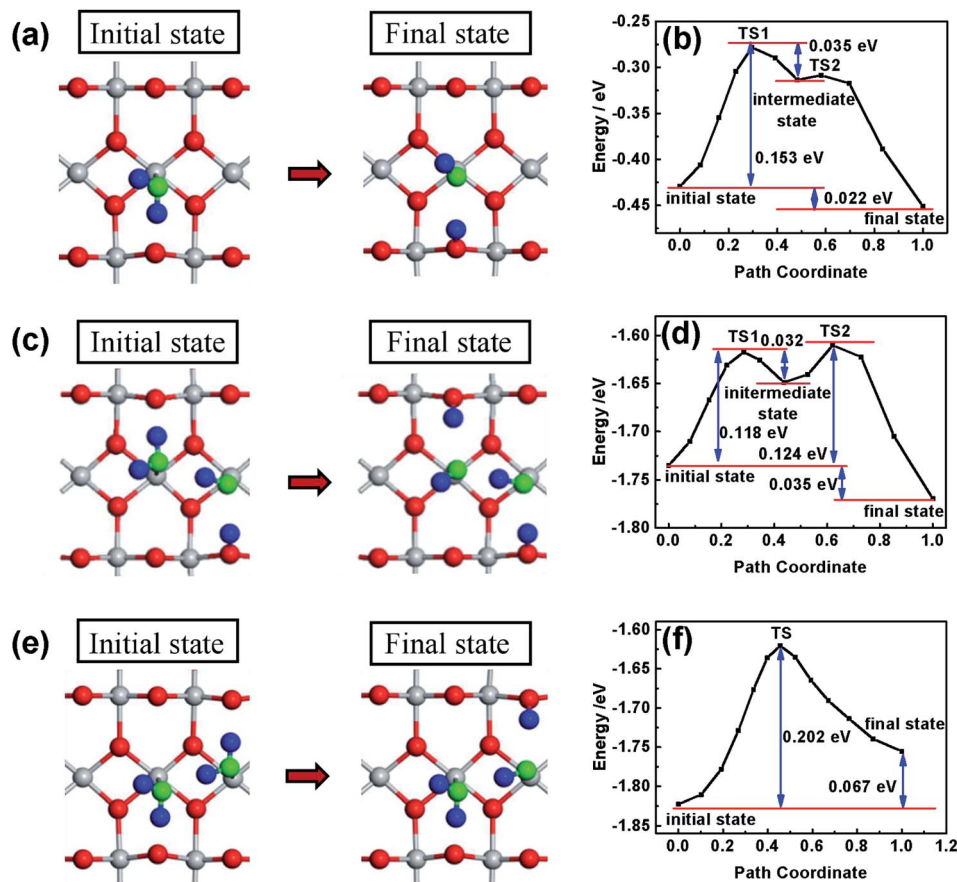
Fig. 4 A slab model of the rutile TiO 2 (110) surface with H 2 O adsorbed on Ti atoms. Grey and red spheres represent the oxygen and titanium atoms from TiO 2 , respectively. Blue and green spheres represent hydrogen and oxygen from H 2 O, respectively. The initial and final states of the first H 2 O molecule dissociated on the TiO 2 (110) surface (a) and the corresponding reaction path (b); the initial and final states of the second H 2 O molecule dissociated on the TiO 2 (110) surface with the dissociated H 2 O molecule (c) and the corresponding reaction path (d); the initial and final states of the second H 2 O molecule dissociated on the TiO 2 (110) surface with non-dissociated H 2 O (e) and the corresponding reaction path (f).
