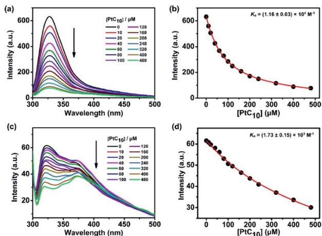
Fig. 1 Fluorescence spectra of CP6A ( 1.0 \times 10^{-5} \text{ M} ) in aqueous PBS (a) pH 7.4 and (c) pH 5.0 recorded in the presence of different concentrations of PtC 10 at 298 K. (b) and (d) nonlinear least-squares analyses used to calculate the K_a value.
