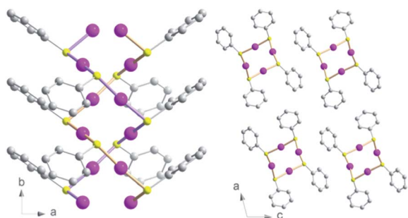
Fig. 1 Views of the crystallographic structure of the [Au(SPh)] n CP along the c axis (left) and b axis (right). Pink, yellow and grey spheres are for gold, sulfur and carbon atoms. Hydrogen atoms are omitted for clarity.
