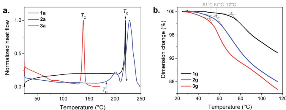
Fig. 4 (a) DSC in air with a heating rate of 10\text{ }^{\circ}\text{C min}^{-1} , of the three amorphous a\text{-[Au(SR)]}_n compounds: 1a (black), 2a (blue) and 3a (red), showing the crystallization temperature ( T_c ) or the decomposition temperature ( T_d ). (b) TMA curves of 1g (black), 2g (blue) and 3g (red) carried out in air with a heating rate of 3\text{ }^{\circ}\text{C min}^{-1} and an applied force of 0.01 N. The grey arrows and the associated temperatures correspond to the onset of the T_g .
