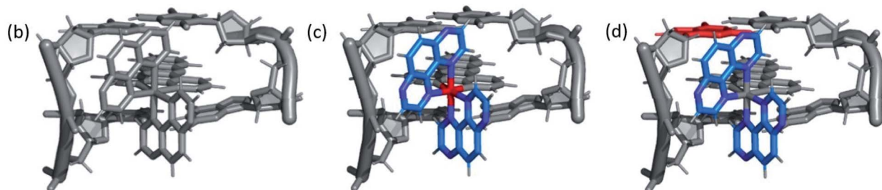
Fig. 4 (a) Equations summarising the excited state electron transfer process of 1 in close proximity to guanine. (b) Schematic example of expected changes in electron density for \Delta - 1 intercalated into a GC/GC base-pair step upon (c) formation of the excited state and (d) subsequent electron transfer. Red = oxidised centre, blue = reduced centre.
