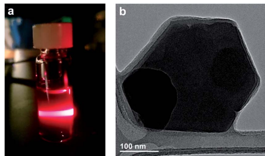
Fig. 4 (a) Photograph of scattered 635 nm light from a suspension of 2-Mo in DMF demonstrating the Tyndall effect. (b) TEM image of a few-layer nanosheet of 2-Mo . Additional images are shown in Fig. S18.†
