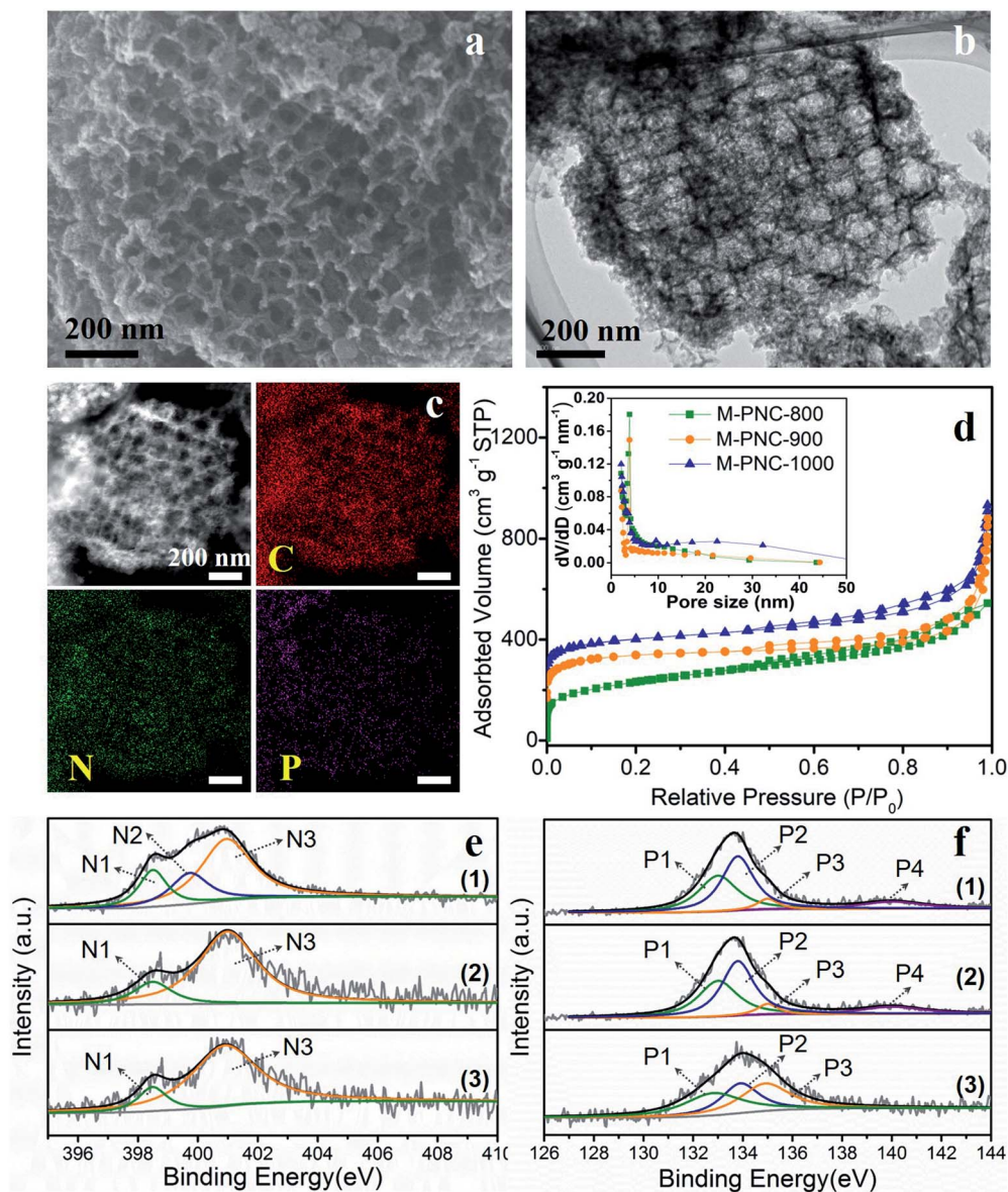
Fig. 2 (a) SEM, (b) TEM, (c) STEM and elemental mapping images of M-PNC-1000. (d) N 2 adsorption–desorption isotherms and pore size distributions of M-PNC- y ( y = 800, 900, 1000); for clarity, the isotherms of M-PNC-900 and M-PNC-1000 were off-set by 70 and 140 cm 3 g -1 . High-resolution XPS spectra of (e) N 1s and (f) P 2p of (1) M-PNC-800, (2) M-PNC-900, (3) M-PNC-1000.
