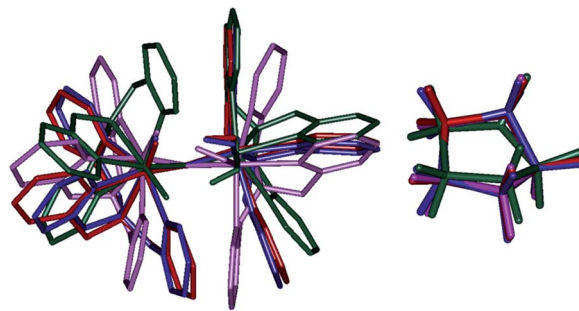
Fig. 10 Structural overlay of ^2\text{RC}_{\text{hs-hs}} (blue), \mathbf{I}^{\text{-}2}\text{TS}_{\text{Hhs-hs}} (red), \mathbf{II}^{\text{-}2}\text{TS}_{\text{Hhs-hs}} (dark green), and \mathbf{III}^{\text{-}2}\text{TS}_{\text{Hhs-hs}} (magenta) and their corresponding cyclopentane ring (right) shown separately. H atoms are omitted for clarity.
