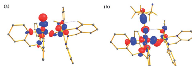
Fig. 9 Computed orbital diagram corresponding to the (a) LUMO of the ^21_{\text{HS-HS}} and (b) HOMO of the \text{I-}^2\text{TS}_{\text{HHS-HS}} .
