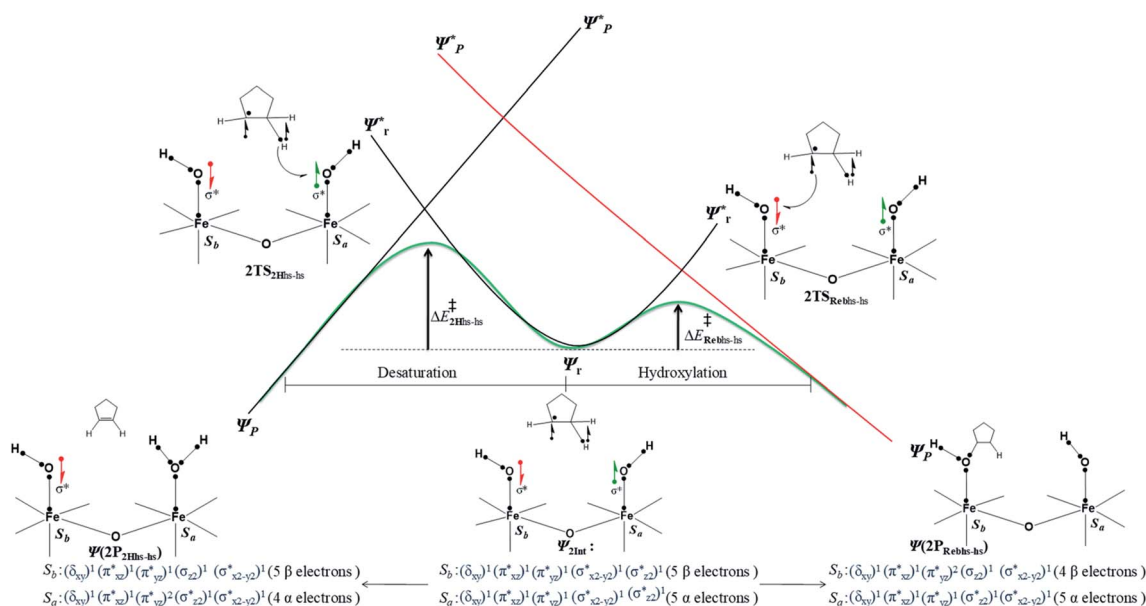
Fig. 11 Valence bond curve crossing diagram for the rebound transition state ( 2 TS rebhs-hs ) (a) and second hydrogen abstraction transition state ( 2 TS 2H 1 hs-hs ) (b) from 2 Int hs-hs . Dots represent valence electrons, and lines implicate chemical bonds.
