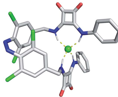
Fig. 2 Calculated structure of the chloride complex 1a^{2-}\text{Cl} (MM+ force field, HyperChem).
