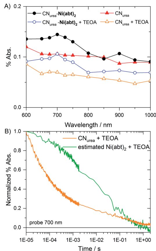
Fig. 6 Temporal evolution of photogenerated reaction intermediates. (A) Transient absorption spectrum of \text{CN}_{\text{urea}} and \text{CN}_{\text{urea}}-\text{Ni}(\text{abt})_2 at 100 \mu\text{s} in pure water and in an aqueous 10 vol% TEOA solution. (B) Normalized kinetics of \text{CN}_{\text{urea}} in TEOA at 700 nm with estimated kinetics of the transfer of charges from carbon-nitride to the co-catalyst. The estimated kinetics were obtained by subtraction of the \text{CN}_{\text{urea}} from \text{CN}_{\text{urea}}-\text{Ni}(\text{abt})_2 kinetics in TEOA and followed normalization. Probed at 700 nm for 355 nm excitation density of 500 \mu\text{J cm}^{-2} .
