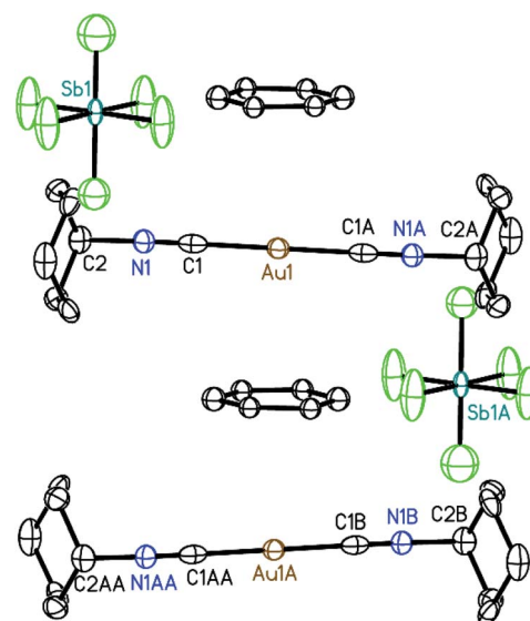
Fig. 5 A portion of the structure of [(C_6H_{11}NC)_2Au](SbF_6) \cdot C_6H_6 ( 7 ) that depicts the sandwich of benzene between two of the gold(I) cations with 50% thermal contours. Hydrogen atoms and the alternate position for the benzene molecules are omitted for clarity.
