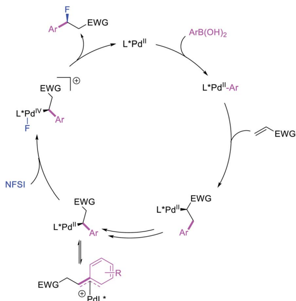
Scheme 28 Mechanism of the 1,1-arylfuorination.
