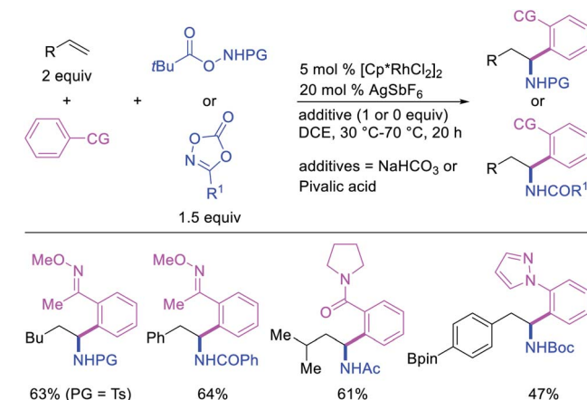
Scheme 20 Rh-catalyzed 1,1-arylamination of alkenes via C–H activation.
