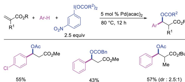
Scheme 22 Pd-catalyzed 1,1-aryloxygenation via C–H activation.
