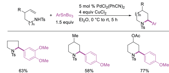
Scheme 18 Pd-catalyzed 1,1-arylamination.
