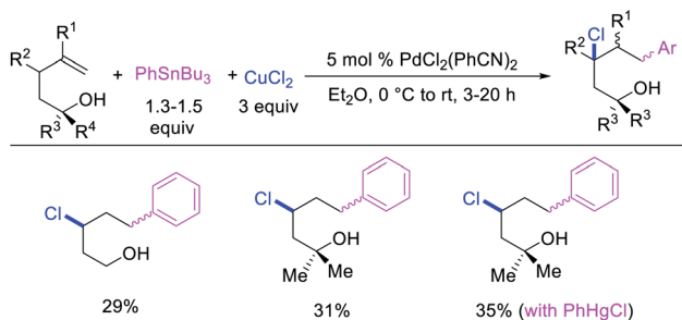
Scheme 56 Pd-catalyzed 1,3-arychlorination.
