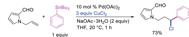
Scheme 19 Pd-catalyzed 1,1-phenylchlorination.
