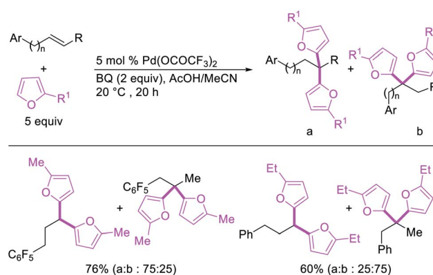
Scheme 6 Pd-catalyzed 1,1-difurylation.
