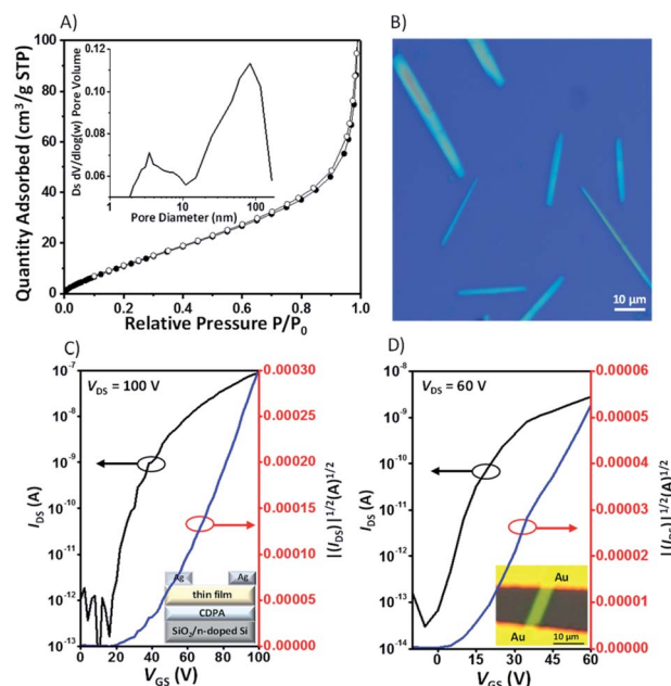
Fig. 8 (A) Nitrogen adsorption (filled symbols) and desorption (open symbols) isotherms at 77 K for 5a (insert: pore size distribution); (B) optical microscopy image of 5a microcrystals from toluene; the representative transfer curves of OFET devices based on the thin film (C) and single-crystal microbelt (D) of 5a measured under N 2 .
