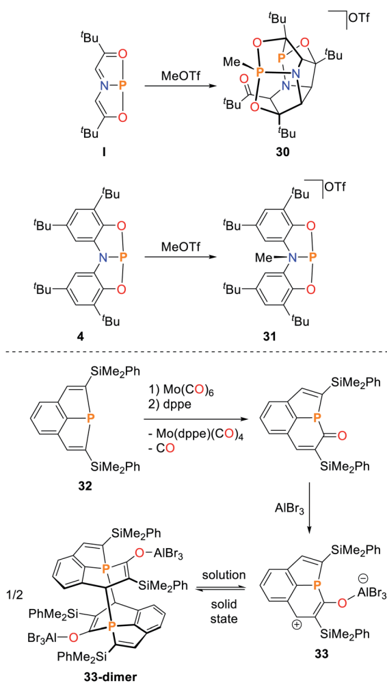
Scheme 14 Reactions of geometrically constrained pnictogen species towards carbon-based nucleophiles, R = \text{Me}, \text{tBu}, \text{Ph} , dppe = diphenylphosphinoethane. 85,92,93
