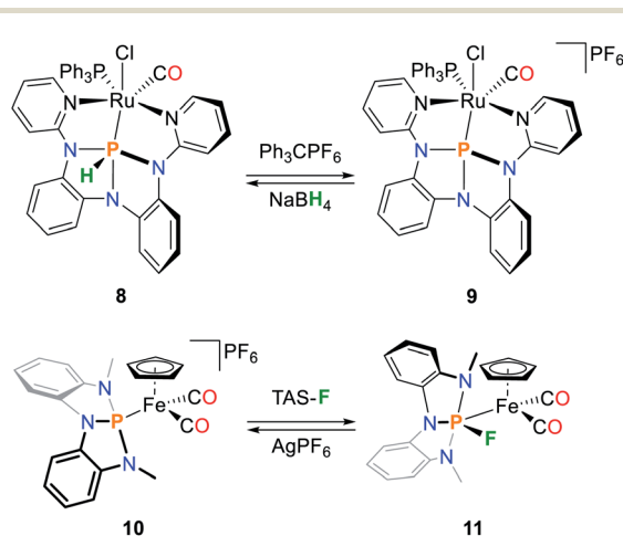
Scheme 5 Reversible P-centered hydride and fluoride addition to transition metal complexes featuring geometrically constrained phosphorus ligands. 69,70
