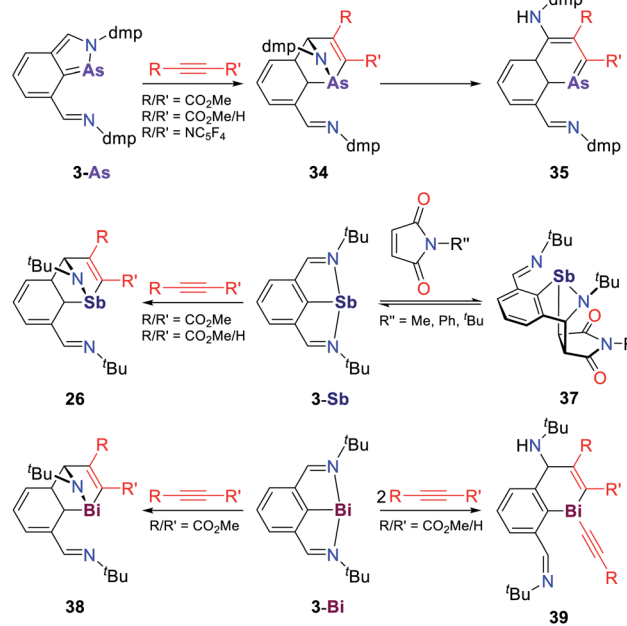
Scheme 15 Reaction of NCN ligated As, Sb and Bi compounds towards electron deficient alkynes and maleimides, dmp = 2,6- \text{Me}_2\text{C}_6\text{H}_3 . 94,95
