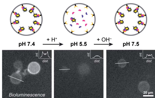
Fig. 3 pH-dependent spatial organization of NanoBiT at the membrane. The bioluminescence of different GUVs was recorded following acidification and subsequent basification of the external solution. GUVs contained DOGS-NTA-Ni (1%), LgBiT and SmBiT ( 5 \mu\text{M} each). \alpha -Hemolysin ( 20 \mu\text{g ml}^{-1} ) facilitated equilibration of the pH over the membrane. The insets display the luminescence intensities along a cross section of the GUVs (indicated by white bars). Note the absence of membrane-associated peaks at acidic pH.
