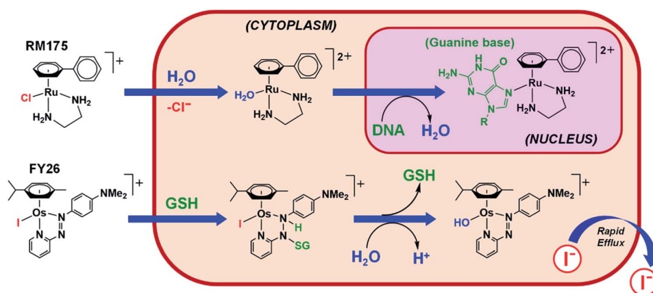
Fig. 4 Hydrolytic activation of two types of half-sandwich complex; RM175 (Ru1), bearing a σ-donor bidentate ligand (en), for which hydrolysis is activated by reduced [Cl − ] levels in cells; FY26 (Os4), bearing a strong π-acceptor ligand (azpy), for which hydrolysis is activated by GSH attack on the azo-bond. 24,29
