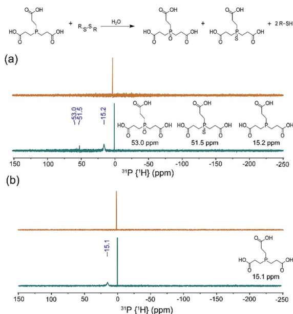
Fig. 5 ^{31}\text{P} ( ^1\text{H} ) NMR spectra in 2HP \beta/S_8 or 2HP \beta solutions incubated with TCEP. (a) 25% w/w solution of 2HP \beta with 500 mg S_8 before (top) and after (bottom) addition of 10 mg TCEP with overnight incubation. (b) 25% w/w 2HP \beta without sulfur in PBS before (top) and after (bottom) TCEP addition and incubation; no oxidized product peaks are observed.
