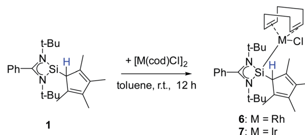
Scheme 6 Synthesis of \{[\text{PhC}(\text{NtBu})_2\text{SiH}(\text{C}_5\text{Me}_4)]\{\text{RhCl}(\text{cod})\} ( 6 ) and \{[\text{PhC}(\text{NtBu})_2\text{SiH}(\text{C}_5\text{Me}_4)]\{\text{IrCl}(\text{cod})\} ( 7 ).
