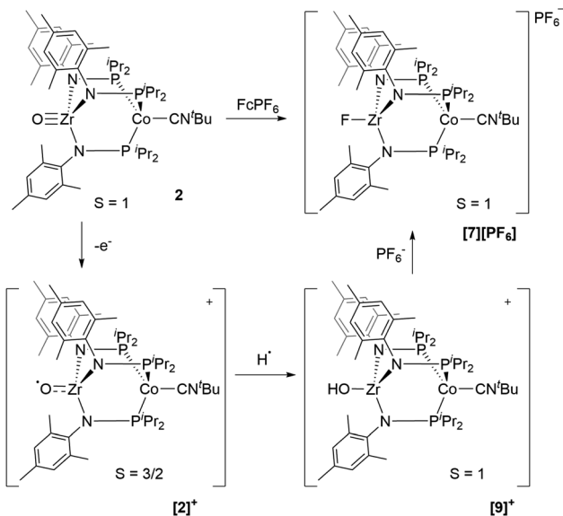
Scheme 5 Proposed transformation from oxo compound 2 to fluoride complex [\text{7}][\text{PF}_6] based on experimental and computational study.
