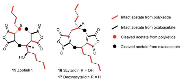
Fig. 3 Incorporation patterns in octadrides and nonadrides from feeding studies with [1,2- 13 C 2 ]-acetate.
