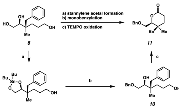
Scheme 4 Synthesis of lactone bearing vicinal quaternary-trisubstituted stereocenters: (a) \text{Bu}_2\text{SnO} , MeOH, reflux, 18 h; (b) BnBr, TBAB, toluene, reflux, 20 h, 60% yield over 2 steps; (c) TEMPO, PIDA, \text{CH}_2\text{Cl}_2 , 23 °C, 18 h, 65% yield.
