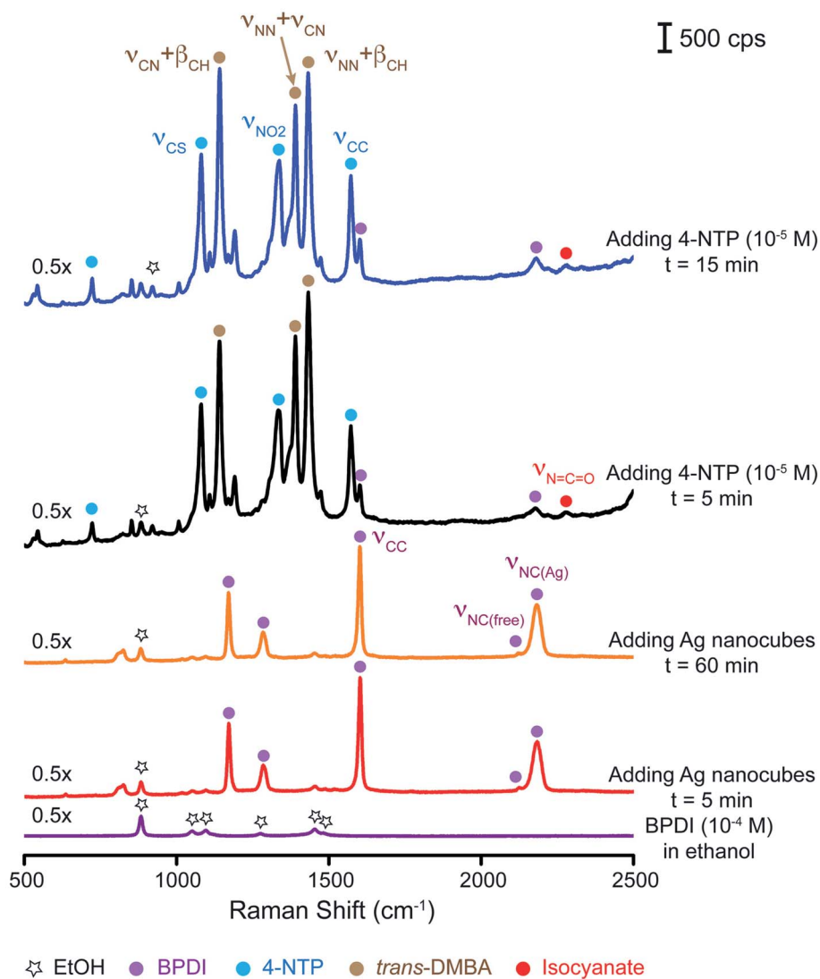
Fig. 5 Raman spectrum recorded from a BPDI solution ( 10^{-4} M) in ethanol and time-elapsing SERS spectra collected at different time points from an ethanolic suspension of Ag nanocubes and BPDI before and after the addition of 4-NTP solution in ethanol ( 10^{-5} M).
