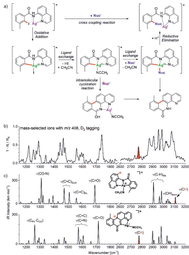
Fig. 10 (a) Silver catalyzed C–Nuc coupling and the mechanism proposed based on ESI-MS and ion spectroscopy study. (b) IR spectrum of ions with m/z 408 isolated from the reaction mixture measured by D_2 -tagging photodissociation method. 55,56 (c) DFT predicted spectra for possible isomers of the detected intermediates with m/z 408. Adapted with permission from ref. 54. Copyright 2018, American Chemical Society.
