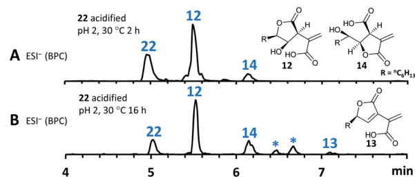
Fig. 8 Lactonization under acidic conditions. (A), ESI - spectrum of 22 (obtained directly via incubation of 20 with SpoG) acidified with formic acid to pH 2, at 30\text{ }^\circ\text{C} for 2 h; (B), as (A), 30\text{ }^\circ\text{C} for 16 h. *Unknown degradation compounds. R = n\text{C}_6\text{H}_{13} .
