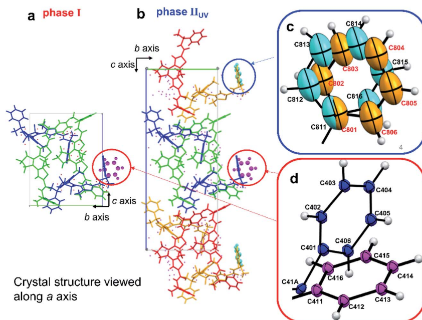
Fig. 4 Crystal structures from the (100) face of (a) phase I and (b) phase \text{II}_{\text{UV}} . (c) Enlarged view of disordered phenyl groups circled in blue. (d) Enlarged view of disordered phenyl groups circled in red.
