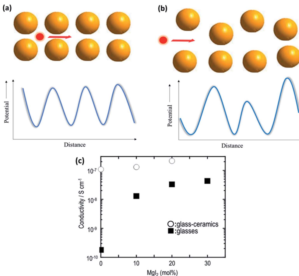
Fig. 8 Potential energy landscape for (a) crystalline and (b) amorphous materials for the transport of ions; (c) plot of ionic conductivity as a function of \text{MgI}_2 concentration in 60\text{MgS-40P}_2\text{S}_5 parent glass. Reproduced from ref. 123 with permission, copyright 2014, Elsevier.
