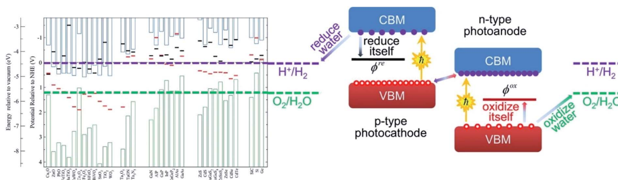
Fig. 1 The relationship between band edge position and self-reduced and/or oxidized potential for various semiconductors. Reprinted with permission from ref. 39. Copyright 2012, American Chemical Society.
